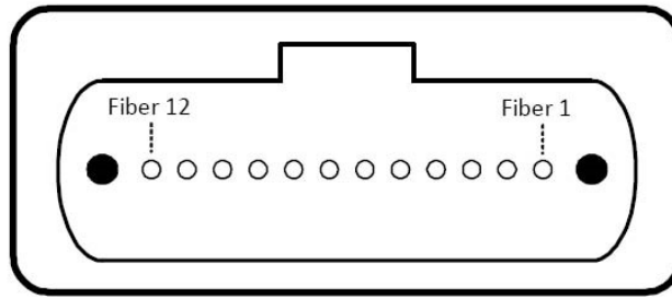
Outside View of the QSFP Module MPO
